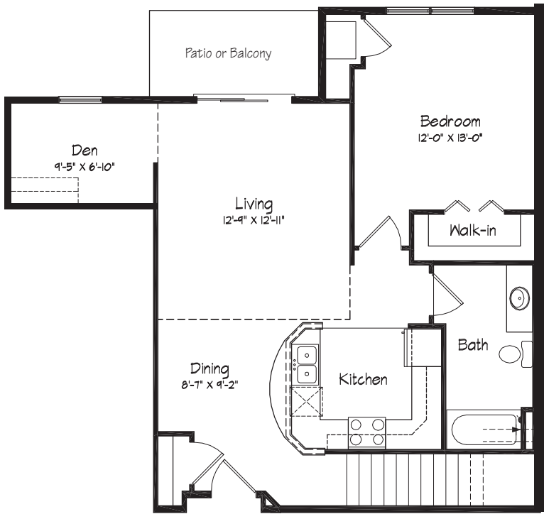
Lower Level
